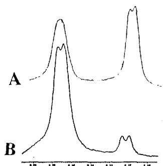
Figure: H-2 proton of ( \pm ) 3 (A) and 3 (B) in the presence of \text{Eu}(\text{hcf})_3 .
