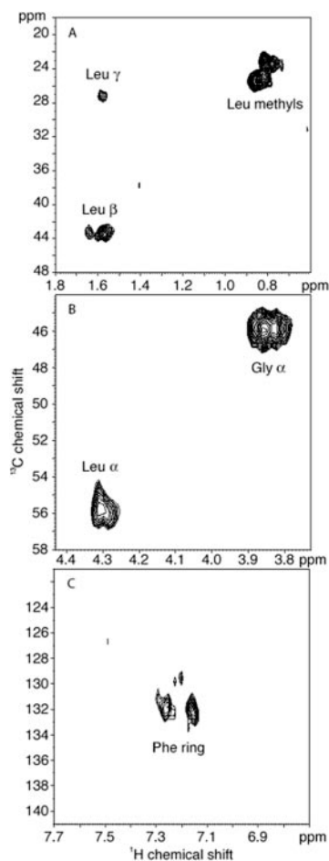
FIG. 5. ^1H - ^{13}C HSQC spectrum of G\alpha protein labeled at Leu-348, Gly-352, and Phe-354. The panels display the regions containing the Leu-348 methyl C\beta -H and C\gamma -H resonances. The Gly-352 (A) and Leu-348 (B) C\alpha -H resonances and the Phe-354- ^{13}C -ring resonances (C).
