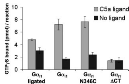
FIG. 3. C5a receptor activation of ligated G proteins. C5a receptors (1–5 nM) in urea-stripped membranes were incubated with C5a ligand (100 nM) and G\alpha proteins (1 \mu M ) and G\beta\gamma (0.5 \mu M ) and GTP \gamma S (3 \mu M ) in 20- \mu l reactions for 10 min at 30 °C and then filtered and counted. Data shown are the average \pm S.E. of six experiments.
