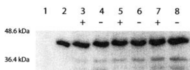
FIG. 2. SDS-PAGE/Western analysis of semisynthetic G\alpha . Ligated product was observed after 24 h. Lane 1, purified G\alpha_{i1}\Delta CT thioester (negative control); lane 2, purified G\alpha_{i1} (N346C). Time points were taken at 24 (lanes 3 and 4), 48 (lanes 5 and 6), and 72 h (lanes 7 and 8) and treated with (+) or without (-) 15 mM dithiothreitol before separation on 10% SDS-polyacrylamide gels. Products were transferred to membranes and blotted with anti-carboxyl-terminal G\alpha_{i1} antibody.
