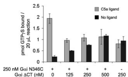
FIG. 4. Competitive inhibition of C5a receptor activation by G\alpha_i\Delta CT . C5a receptors (1–5 nM) in urea-stripped membranes were incubated with C5a ligand (100 nM) and G\alpha_i N346C proteins (250 nM) and G\beta\gamma (0.5 \mu M ) and GTP\gamma S (3 \mu M ) in 20- \mu L reactions. Indicated amounts of G\alpha_i\Delta CT were added, and reactions proceeded for 10 min at 30 °C and then filtered and counted. Data shown are the average \pm S.E. of three experiments.
