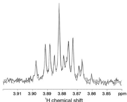
FIG. 7. One-dimensional ^1\text{H} spectra of the G\alpha protein before and after the addition of \text{AlF}_4^- . The spectra are virtually identical, indicating that there is no overall change in the mobility of the protein due to the binding of \text{AlF}_4^- . The changes in the carboxyl-terminal region of the protein are dramatic and localized.
