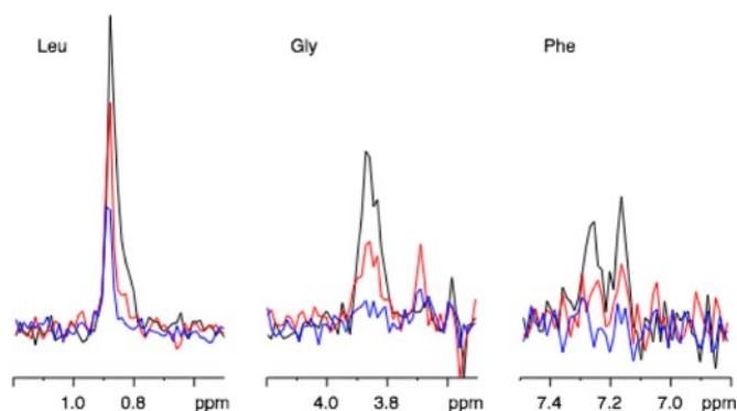
FIG. 6. Intensity of the HSQC NMR resonances as a function of added AlF_4^- . Slices from the two-dimensional HSQC spectra at different concentrations of AlF_4^- . Black line is spectra obtained with no additional AlF_4^- . Red indicates two molar equivalents of AlF_4^- . Blue represents four molar equivalents of AlF_4^- .
