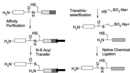
FIG. 1. Expressed protein ligation. G_{\alpha_1}\Delta CT (white box) is expressed in E. coli as a fusion protein, G_{\alpha_1}\Delta CT-intein-CBD. The chitin-binding domain (CBD; gray box) allows affinity purification on the chitin matrix (black arrow). Intein domain (diagonal lines) catalyzes N→S acyl transfer. Incubation with mercaptoethanesulfonic acid results in cleavage of the target protein from the intein-CBD domains, generating recombinant G_{\alpha_1}\Delta CT thioester. The thioester protein thereafter undergoes native chemical ligation with CNLKDCGLF peptide (cross-hatched).
